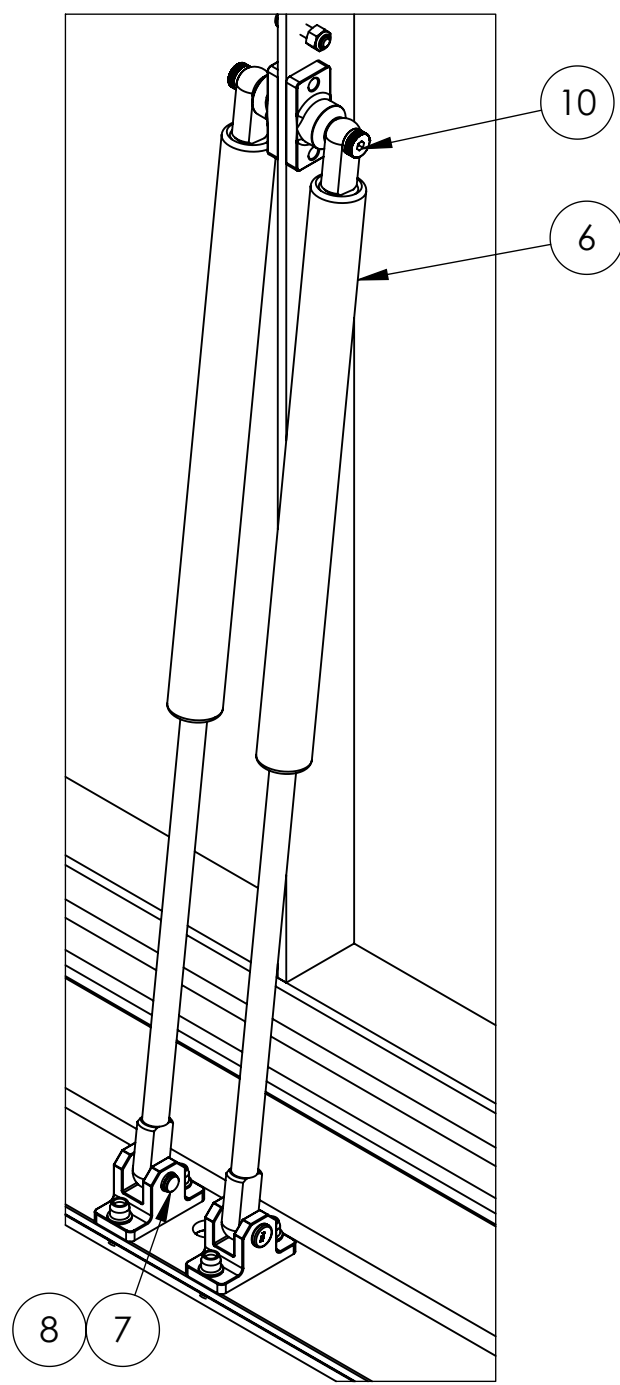
DETAIL W SCALE 1 : 4
