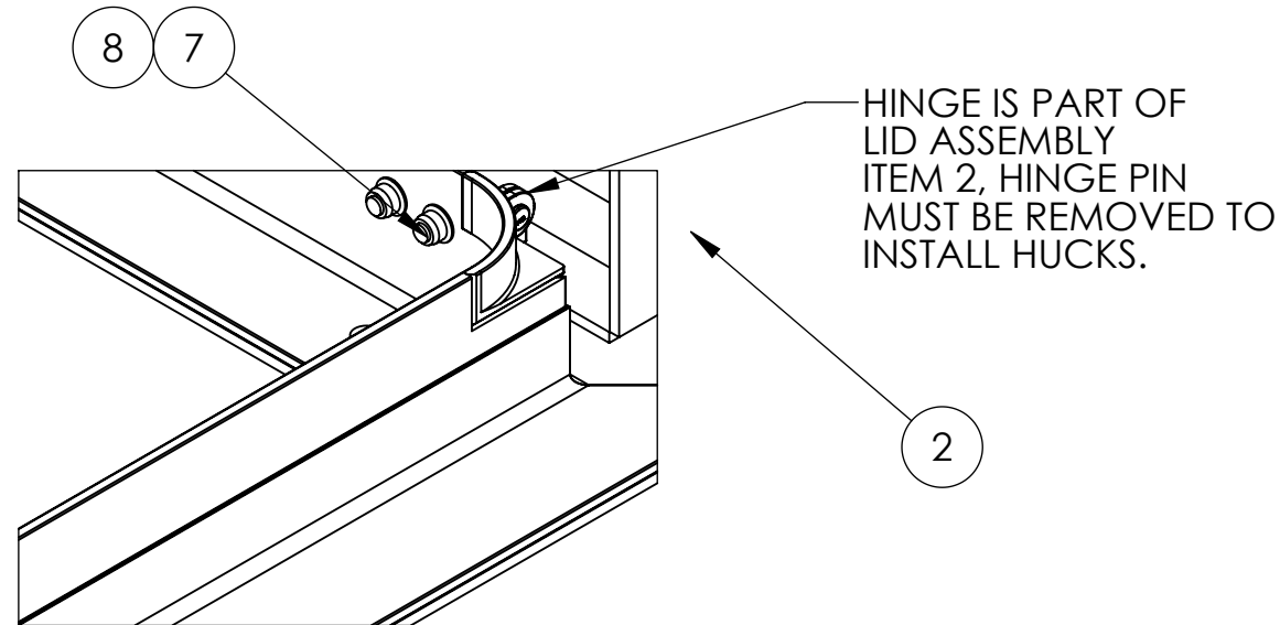
DETAIL F SCALE 1 : 4
