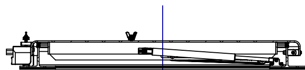
SECTION N-N
