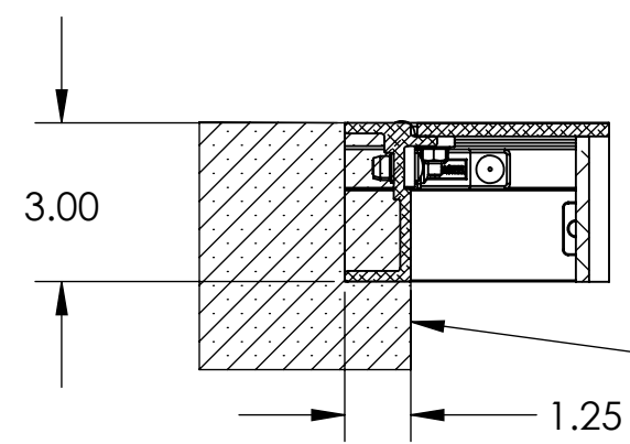
SECTION H-H SCALE 1 : 4
